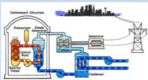
Fig 1: Schematic diagram of a nuclear power plant
